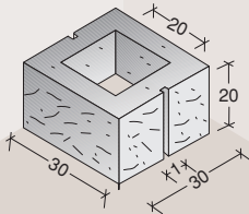
m split 30 x 30 x 20
